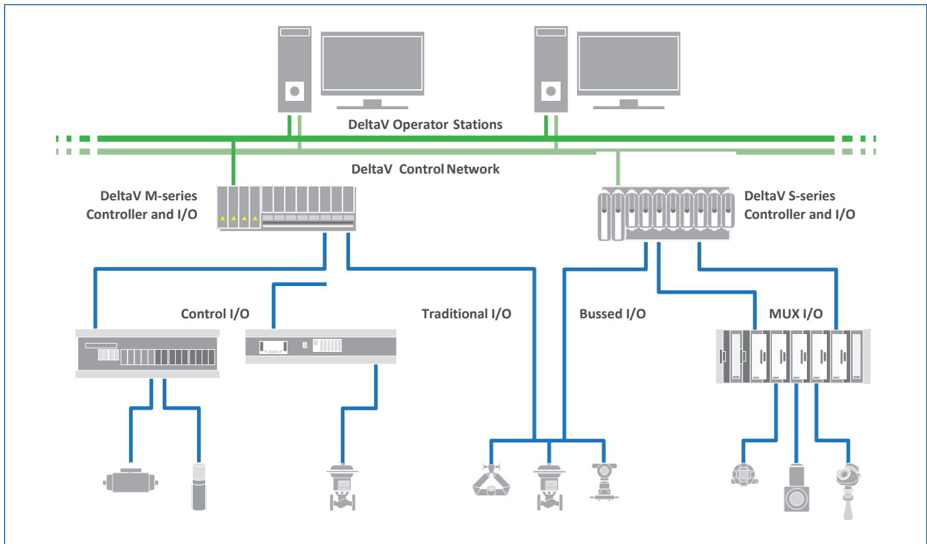
FlexConnect™ Solutions for PROVOX™ MUX I/O.
