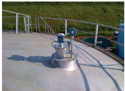
Figure 3.4: Manways are normally located near the tank wall which provides mechanical stability.
