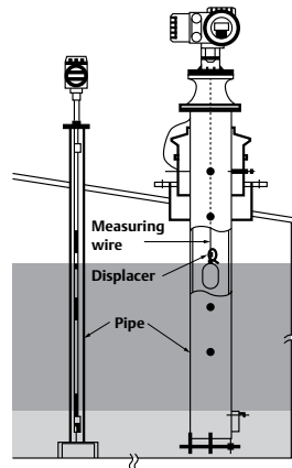
Figure 2.7: Servo gauge and temperature sensor measuring inside still-pipes.
